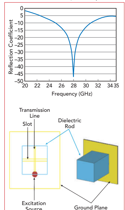
▲ Fig. 1 Magnitude of the input reflection coefficient of the individual DRA element (the illustration shows the configuration of the radiating structure).
