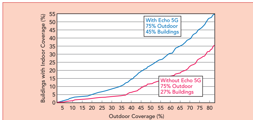
▲ Fig. 8 Outdoor vs. indoor coverage, urban, without Echo (red) and with Echo (blue).
