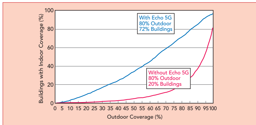
▲ Fig. 9 Outdoor vs. indoor coverage, suburban, without Echo (red) and with Echo (blue).
