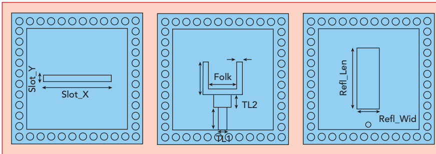
▲ Fig. 2 Antenna element feeding structure.
