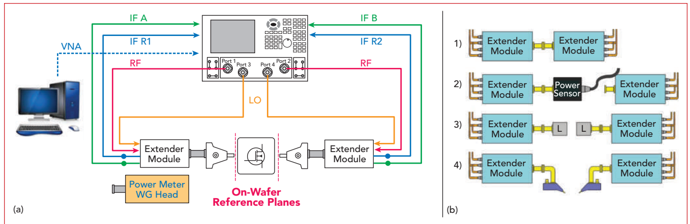
Fig. 3 Conventional mmWave measurement using waveguide extenders with a 4-port, two-source VNA (a) and the four-step calibration procedure (b).
