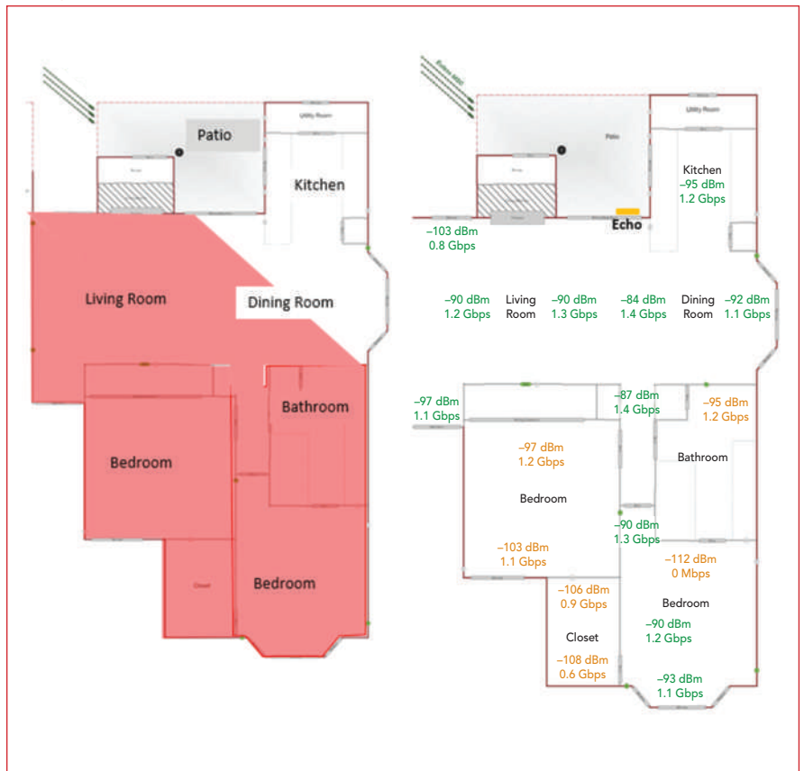
▲ Fig. 7 Suburban apartment trial results, before and after Echo 5G deployment.
